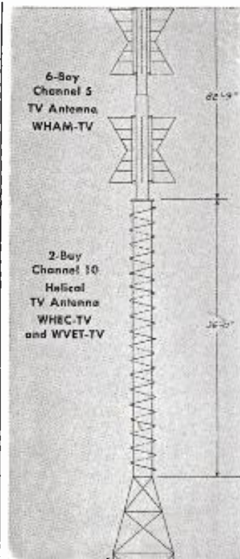
This General Electric engineer's drawing illustrates the proposed VHF Helical Antenna installation at Rochester.
